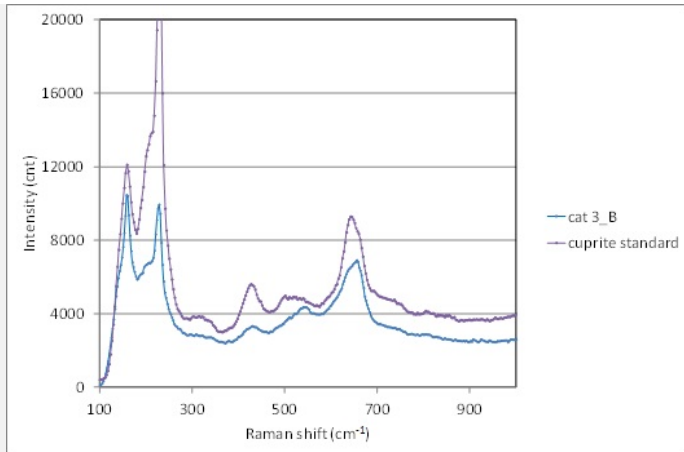
Fig. 9: Raman spectrum of the red-orange inner corrosion layer (CP2) of the external side (cat3_B) compared to a cuprite standard spectrum. Settings: laser wavelength 532nm, acquisition time 100s, one accumulation, filter D2 (0.75-0.8 mW), hole 500, slit 80, grating 600. Method of analysis: Raman spectroscopy, Lab Swiss National Museum, Affoltern a. Albis ZH,
