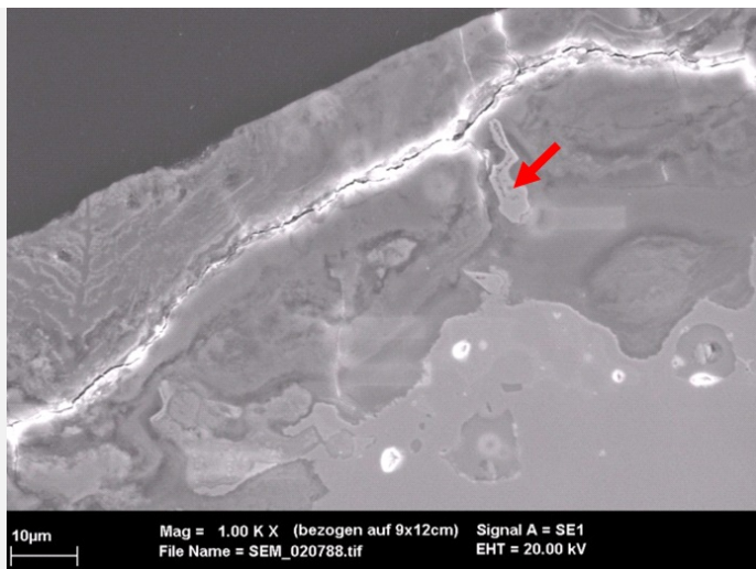
Fig. 7: SEM image of the metal sample (detail of Fig. 5, reversed picture), SE-mode. From bottom right to top left: the metal, the inner and outer corrosion layers separated by a large fissure. The red arrow indicates a remnant of the Sn-rich alpha-delta eutectoid,
