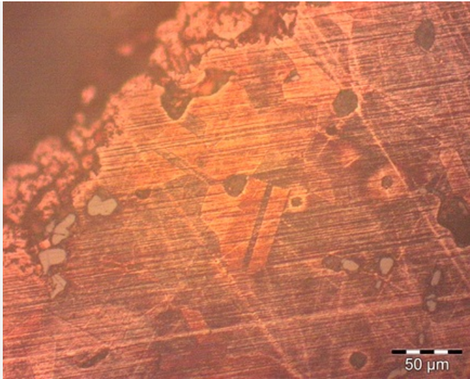
Fig. 9: Micrograph of a selected area of the metal sample showing grains and twin lines,
