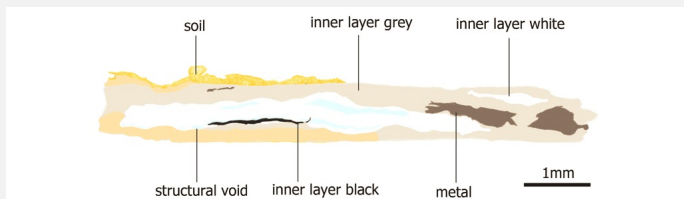
Fig. 16: Improved representation of the stratigraphy of corrosion layers of the military tag from visual observations and analyses,
