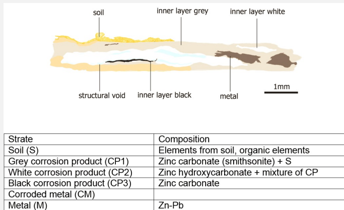
Fig. 16: Improved representation of the stratigraphy of corrosion layers of the military tag from visual observations and analyses,
