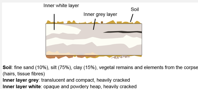
Fig. 3: Stratigraphic representation of fragment b of the military tag in cross-section by macroscopic observation,
