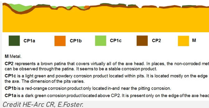
Fig. 8: Stratigraphic representation of corrosion products of the axe head (based on visual observations),
