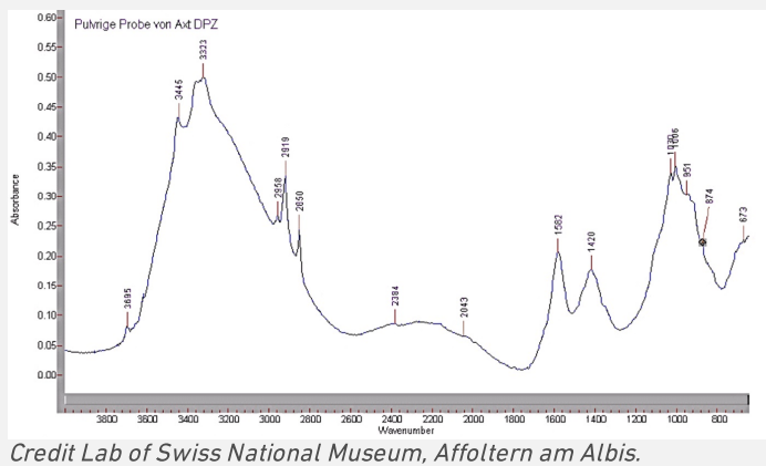
Fig. 17: FTIR spectrum of sample 4 (white particle),
