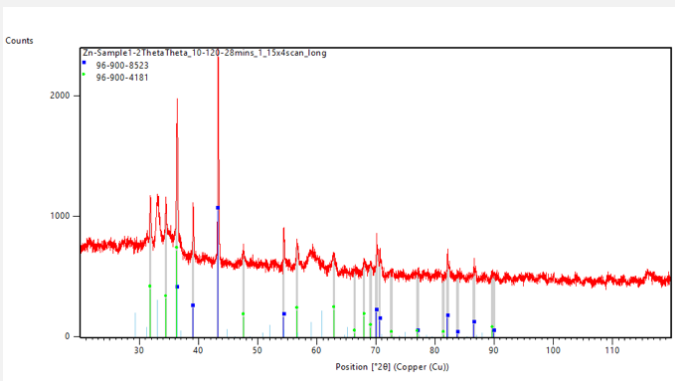
Fig. 13: XRD-spectrum for the analysis of powder sample 1. Ref. 96-900-8523 (in blue) corresponds to pure zinc and 96-900-4181 (in green) to zincite (ZnO),
