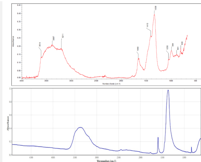
Fig. 10: FTIR spectrum (ATR mode) of the white corrosion product (top), and of synthesized copper nitrate ( \text{Cu}(\text{NO}_3)_2 \cdot 3\text{H}_2\text{O} ) (bottom),
