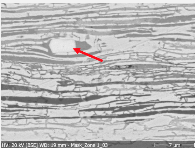
Fig. 5: SEM image (BSE-mode) of the metal sample from Fig. 4 (detail), the elongated grains are the result of repeated hammering. Absence of strain lines indicates that the metal is annealed. The darker areas are Cu-rich phases and the lighter areas are Ag-rich phases. The arrow shows an As- and Pb inclusion,
