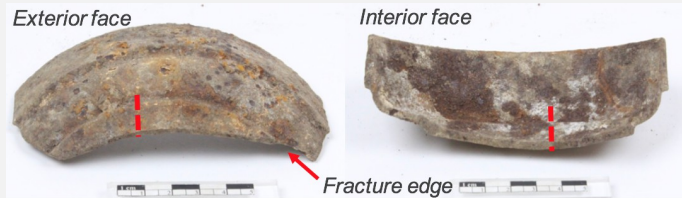
Fig. 2: The exterior and interior faces before sampling. The dotted line represents the sample location (a cross-section of the metal). The fracture edge corresponds to the edge that was formerly attached to the remaining artefact,
