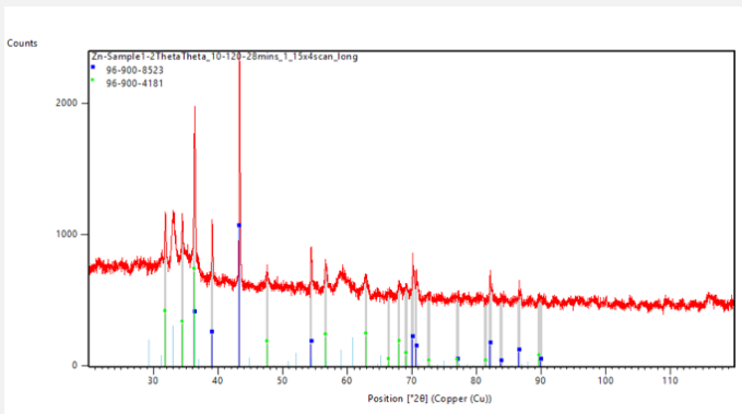
Fig. 12: XRD-spectrum for the analysis of powder sample 1. Ref. 96-900-8523 (in blue) corresponds to pure zinc and 96-900-4181 (in green) to zincite (ZnO),
