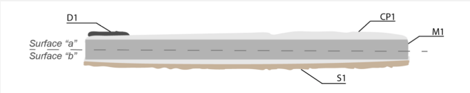
Fig. 3: Schematic presentation of the artefact based on visual macroscopic observation. CP = corrosion product, D = deposit, M = metal, S = soil,
