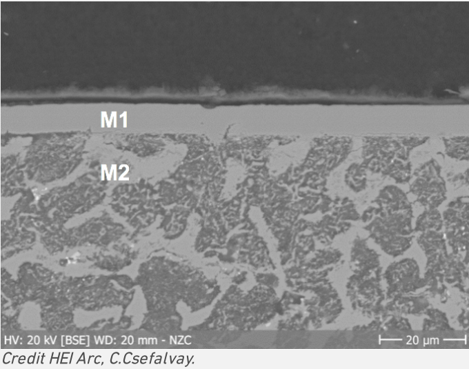
Fig. 5: SEM-image (BSE-mode) of a selected area from Fig. 4 (detail), showing the metal plating (M1) and the bulk metal (M2),
