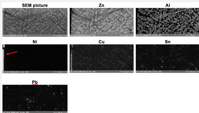
Fig. 9: SEM image and elemental chemical distribution of the selected area from Fig. 7 (rotated 270° and inverted). Method of analysis: SEM-EDS. Lab. of Electronic Microscopy and Microanalysis, Néode, HEI Arc,
