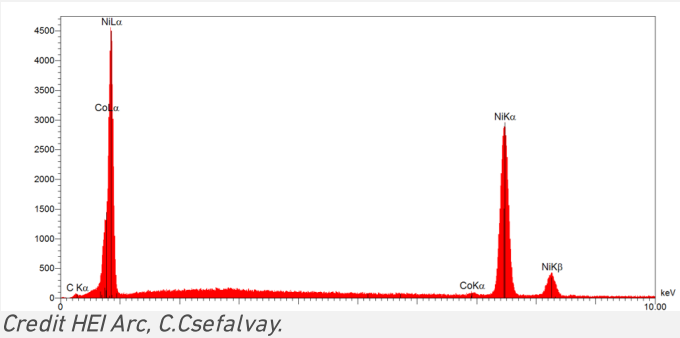
Fig. 6: EDS-spectrum showing the chemical composition of the metal plating (M1). Method of analysis: SEM-EDS. Lab. of Electronic Microscopy and and Microanalysis, Néode, HEI Arc,
