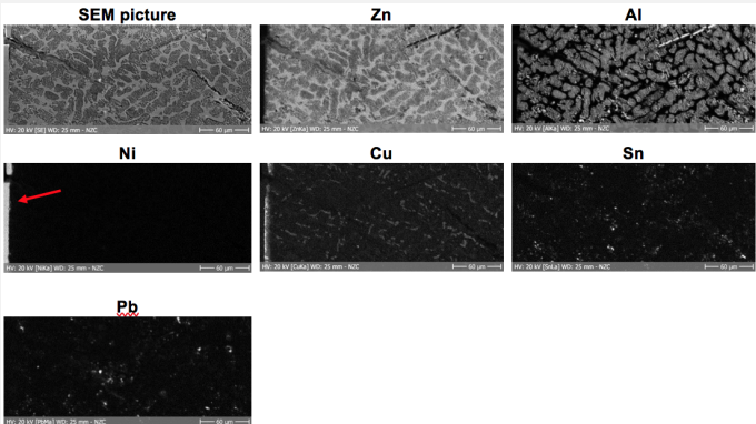
Fig. 9: SEM image and elemental chemical distribution of the selected area from Fig. 7 (rotated 270° and inversed). Method of analysis: SEM-EDS. Lab. of Electronic Microscopy and Microanalysis, Néode, HEI Arc,
