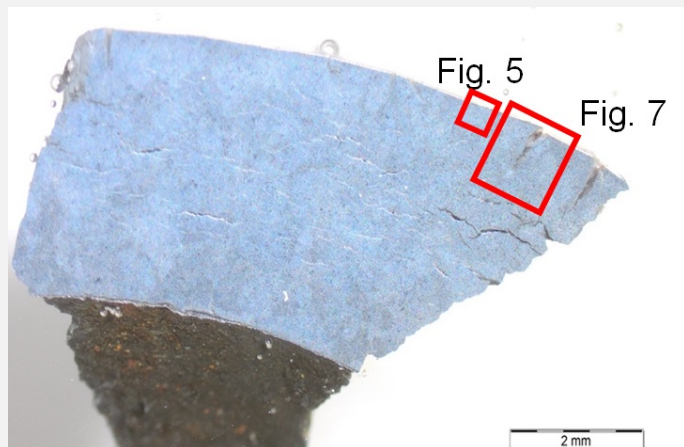
Fig. 4: Micrograph of the cross-section of the sample taken from the domed cap nut showing the locations of Figs. 5 and 7,
