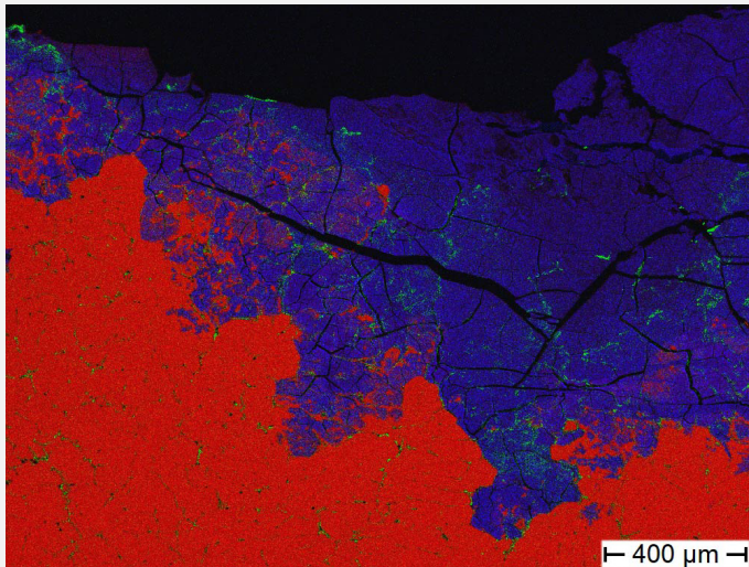
Fig. 12: Al (red), O (blue) and Cu (green) distribution of the area of Fig. 11. Method of analysis: SEM-EDS. Lab. of Electronic Microscopy and Microanalysis, Néode, HEI Arc,
