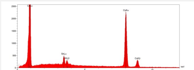
Fig. 15 : EDS spectrum of the dendritic phase,
