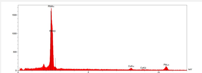
Fig. 17: EDS spectrum of Pb nodules,
