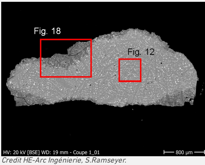
Fig. 11: SEM image of the cross-section similar to Fig. 9, BSE-mode. The area selected for elemental chemical analysis (Fig. 12) is marked by a rectangle. Fig. 18 is similarly indicated,
