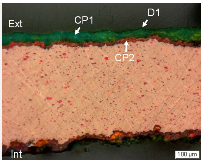
Fig. 6: Micrograph of the metal sample from Fig. 3 and corresponding to the stratigraphy of Fig. 10, polarised light. External side: the regular corrosion crust with outer green, inner red-orange corrosion products and intermediate dark-red corrosion products. Internal side: the irregular corrosion crust with inner red-orange and outer dark-red corrosion products,
