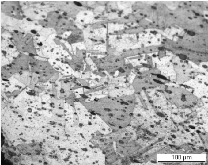
Fig. 5: Micrograph of the metal sample from Fig. 3 (detail), etched, bright field. The metal shows a structure of polygonal and twinned grains. Cuprite inclusions appear as dark spots, and elongated inclusions are visible.
