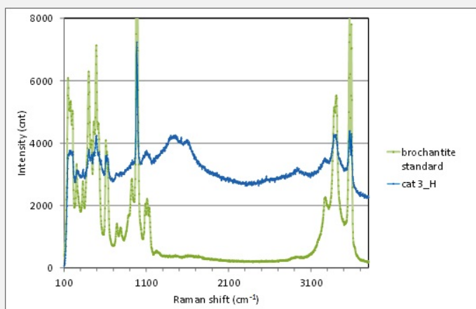
Fig. 9: Raman spectrum of the green outer corrosion layer (CP1) of the external side (cat3_H) compared to a brochantite standard spectrum. Settings: laser wavelength 532nm, acquisition time 100s, one accumulation, filter D2 (0.75-0.8 mW), hole 500, slit 80, grating 600. The peak indicated with an arrow on the cat3_H spectrum is due to fluorescence. Method of analysis: Raman spectroscopy, Lab Swiss National Museum, Affoltern a. Albis ZH,
