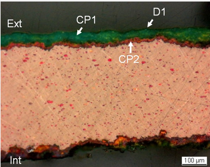
Fig. 6: Micrograph of the metal sample from Fig. 3 and corresponding to the stratigraphy of Fig. 10, polarised light. External side: the regular corrosion crust with outer green, inner red-orange corrosion products and intermediate dark-red corrosion products. Internal side: the irregular corrosion crust with inner red-orange and outer dark-red corrosion products,
