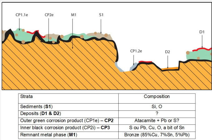
Fig. 16: Improved stratigraphic representation of the headrest from visual observations and analyses (additional mention e or i within the coding correspond to strata in contact with the environment (e) and internal strata (i),
