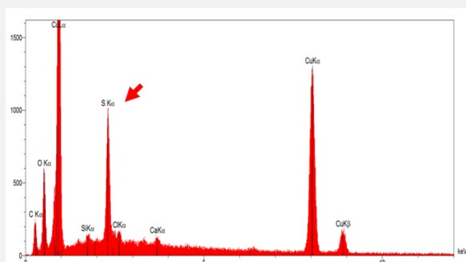
Fig. 14: EDS analysis of the black corrosion powder (Fig. 2). Method of analysis: SEM-EDS, Lab of Electronic Microscopy and Microanalysis, IMA (Néode), HEI Arc,
