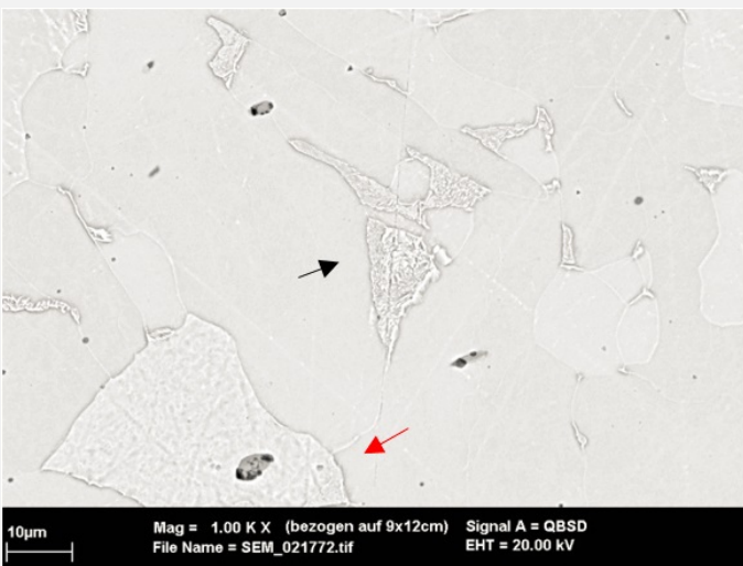
Fig. 7: SEM image of the metal sample from Fig. 3 (detail), BSE-mode, nital etched, bright field. The white ferrite grains contain lamellar pearlite (black arrow) and lenticular grey MnS inclusions (red arrow) in between the grain boundaries,
