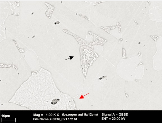
Fig. 7: SEM image of the metal sample from Fig. 3 (detail), BSE-mode, nital etched, bright field. The white ferrite grains contain lamellar pearlite (black arrow) and lenticular grey MnS inclusions (red arrow) in between the grain boundaries,
