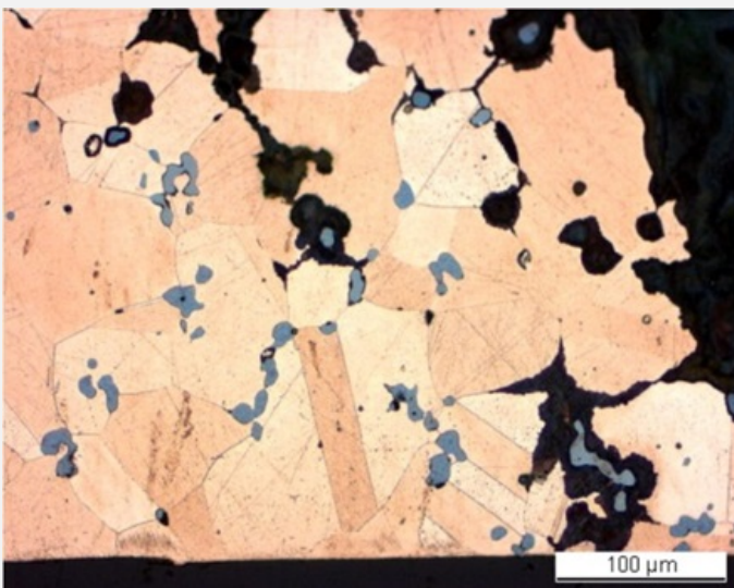
Fig. 5: Micrograph of the metal sample from Fig. 3 (same as Fig. 4), etched, bright field. In pink the metal with few twins, in black the resin and the corrosion products, in light-blue the copper sulphide inclusions,
