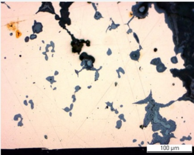
Fig. 4: Micrograph of the metal sample from Fig. 3 (detail), unetched, bright field. In pink the metal, in light-blue the copper sulphide inclusions and in dark-blue corrosion products,
