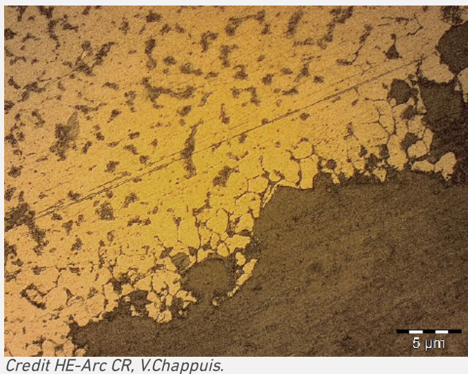
Fig. 8: Micrograph of the selected area of Fig. 7, Nital etched with no clear grain structure, bright field, Intergranular corrosion and grey phase (perlite?) are observed,
