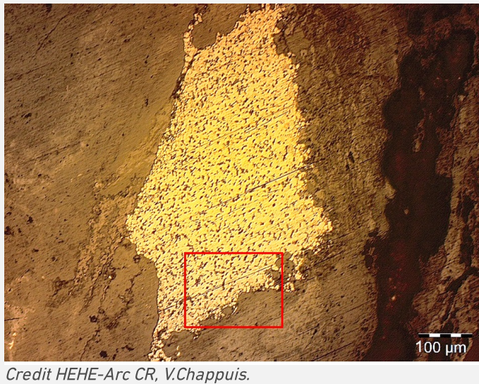
Fig. 7: Micrograph of the metal sample from Fig. 5 (detail, rotated 90°), Nital etched, bright field, with indication of Fig. 8 (red rectangle)
