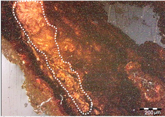
Fig. 9: Micrograph of the metal sample from Fig. 4, bright field. The delimited zone shows what could be leather pseudomorphic fibers filling a void,
