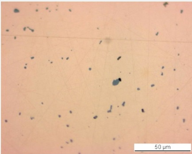
Fig. 5: Micrograph of the metal sample from Fig. 4 (detail), unetched, bright field. Grey copper sulphide inclusions are clearly visible,
