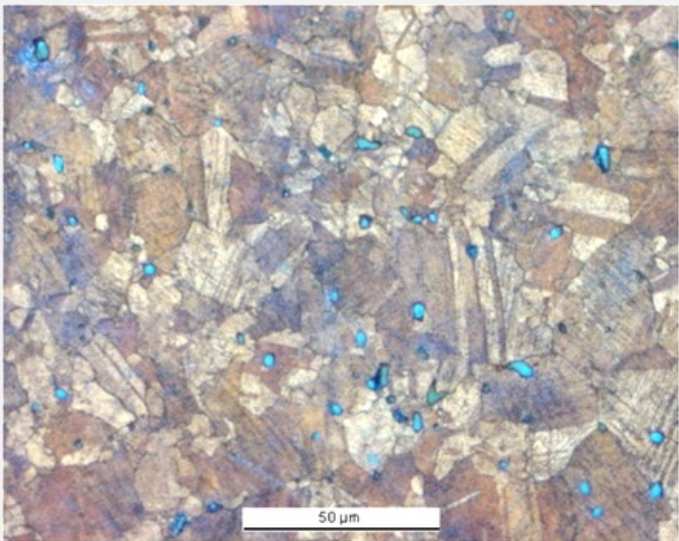
Fig. 6: Micrograph of the metal sample from Fig. 4 (detail), etched, bright field. Small angular re-crystallised grains (some with twins) with slip lines are observed. Copper sulphide inclusions appear in blue,
