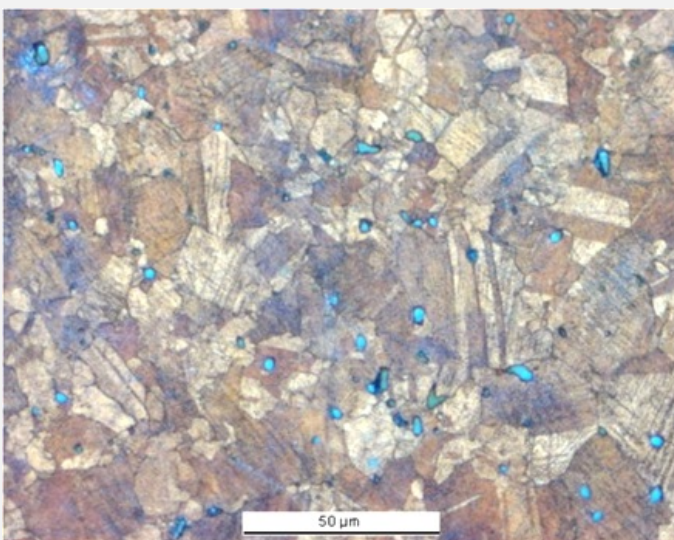
Fig. 6: Micrograph of the metal sample from Fig. 4 (detail), etched, bright field. Small angular re-crystallised grains (some with twins) with slip lines are observed. Copper sulphide inclusions appear in blue,
