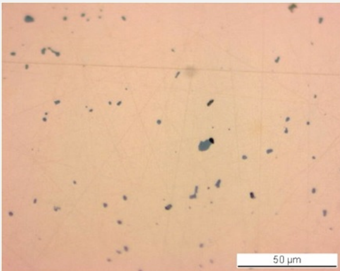
Fig. 5: Micrograph of the metal sample from Fig. 4 (detail), unetched, bright field. Grey copper sulphide inclusions are clearly visible,
