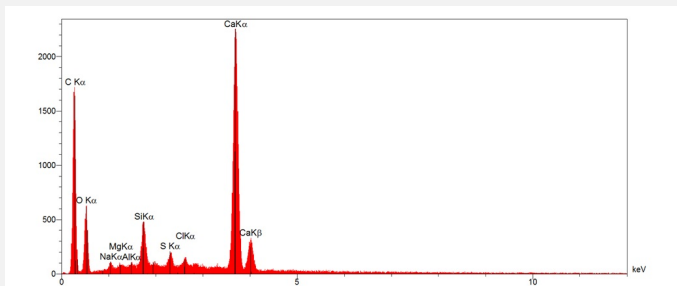
Fig. 11: EDS spectrum of area 4 of Fig. 6,
