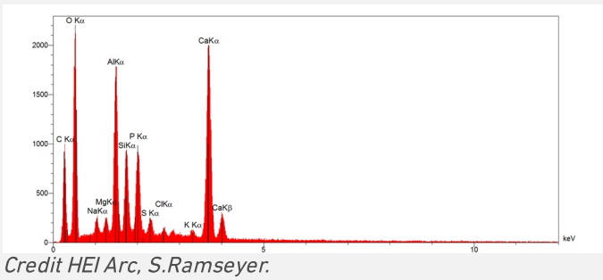
Fig. 8: EDS spectrum of area 2 of Fig. 6,
