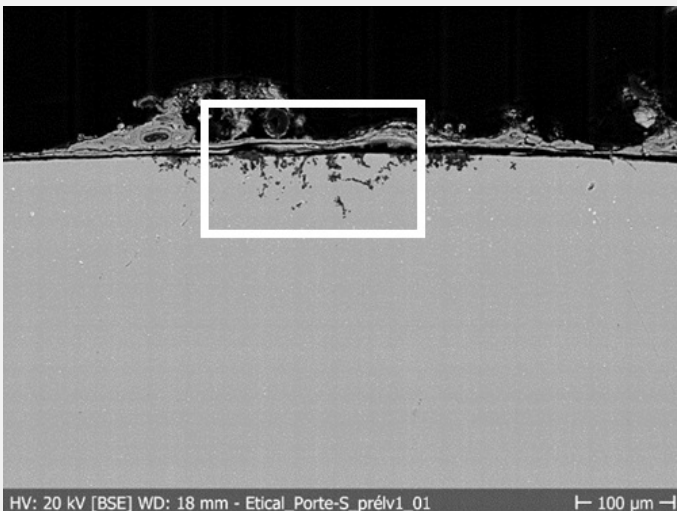
Fig. 3: SEM image of the cross-section of the fragment sampled from the towel bar showing the location of Fig. 4,
