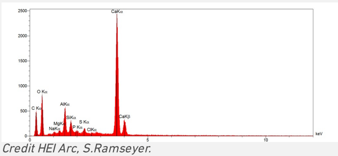
Fig. 7: EDS spectrum of area 1 of Fig. 6,
