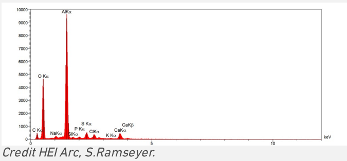
Fig. 9: EDS spectrum of area 3 of Fig. 6,
