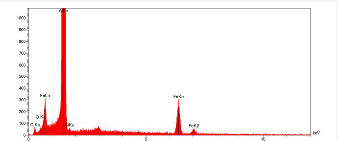
Fig. 5: EDS spectrum of the inclusions of Fig. 4,
