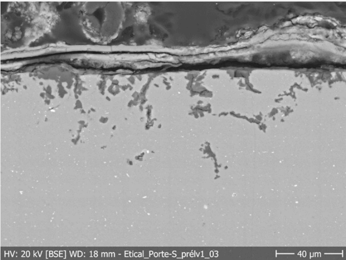
Fig. 4: SEM image of the metal sample from Fig. 3 (detail), BSE-mode. We observe the presence of numerous inclusions,
