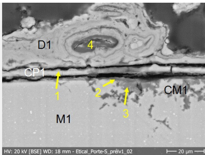
Fig. 6: SEM picture with location of EDS analyses of areas 1 to 4, BSE-mode. From bottom to top: the metal (M1) in light grey, the corroded metal (CM1), CP1 and D1. It can be compared to the stratigraphy representation of Fig. 12,
