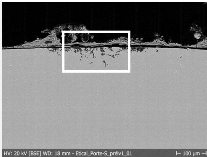
Fig. 3: SEM image of the cross-section of the fragment sampled from the towel bar showing the location of Fig. 4,
