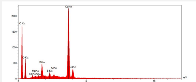
Fig. 11: EDS spectrum of area 4 of Fig. 6,
