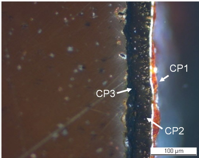
Fig. 8: Micrograph of the same area as Fig. 7 and corresponding to the stratigraphy of Fig. 10, polarized light. From left to right: metal (in brown) covered with a corrosion crust consisting of a black layer, an intermediate brown layer with bright spots, a crack (white line) and a red layer with white particles,
