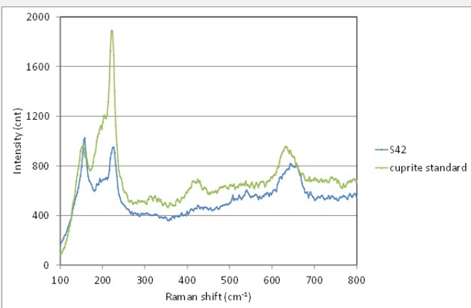
Fig. 10: Raman spectrum of a red-orange corrosion particle (S42) of Fig. 7 compared to the cuprite standard spectrum. Settings: laser wavelength 532nm, acquisition time 10s, one accumulation, filter D2 (0.75-0.8mW), hole 500, slit 80, grating 600. Method of analysis: Raman spectroscopy, Lab of Swiss National Museum, Affoltern a. Albis ZH,
