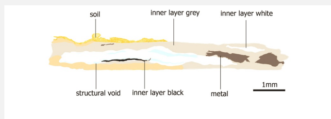
Fig. 18: Improved representation of the stratigraphy of corrosion layers of the military tag from visual observations and analyses,
