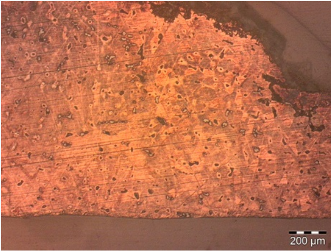
Fig. 7: Micrograph of the metal sample from Fig. 4 showing a dendritic structure and grains,
