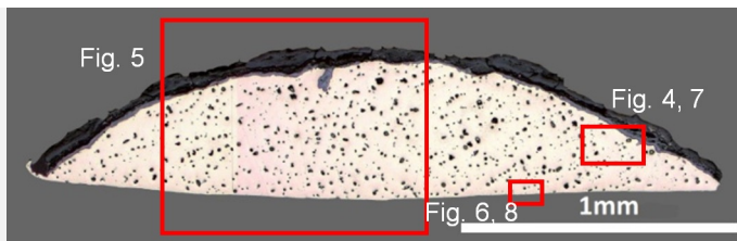
Fig. 3: Micrograph of the cross-section of the sample taken from the bracelet with round diameter showing the location of Figs. 4 to 8,
