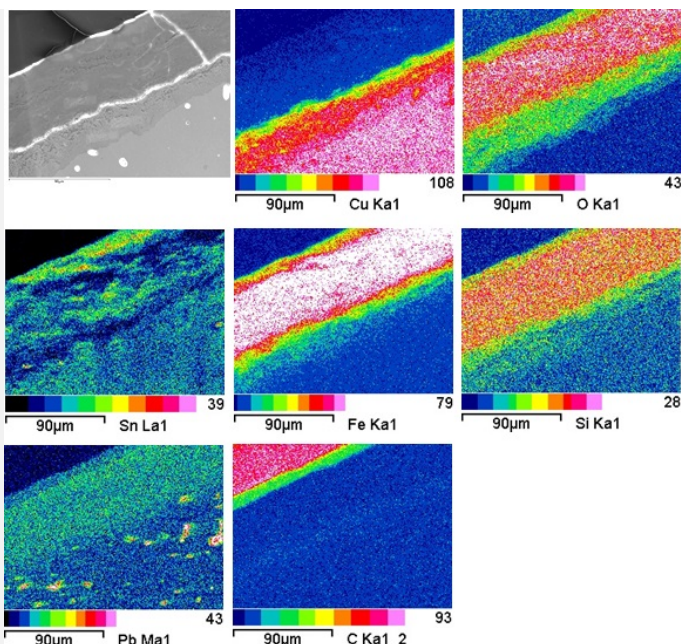
Fig. 8: SEM image, SE-mode, and elemental chemical distribution of a selected area of Fig. 6. The Pb mapping includes the Pb and copper sulphide inclusions, because of a peak interference. Method of examination: SEM/EDS, Laboratory of Analytical Chemistry, Empa,
