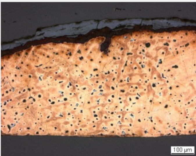
Fig. 5: Micrograph of the metal sample from Fig. 3 (detail), etched, bright field. The dendritic structure is revealed with dark-grey lead inclusions and porosities (in black),
