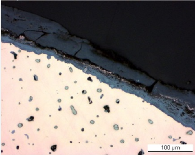
Fig. 4: Micrograph of the metal sample from Fig. 3 (detail), unetched, bright field. In pink the metal with porosity (black), light-grey lead inclusions and dark-grey copper sulphide inclusions,
