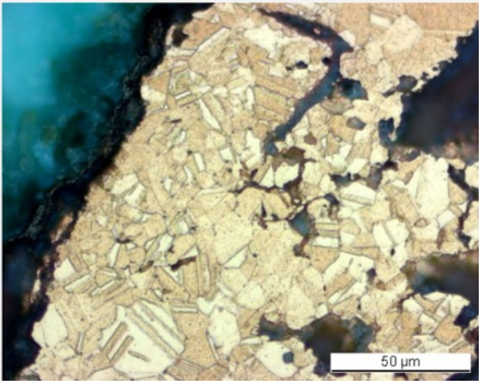
Fig. 5: Micrograph of the metal sample from Fig. 3 (detail of Fig. 4), etched, bright field. The metal shows a structure of mostly small polygonal grains with twins,
