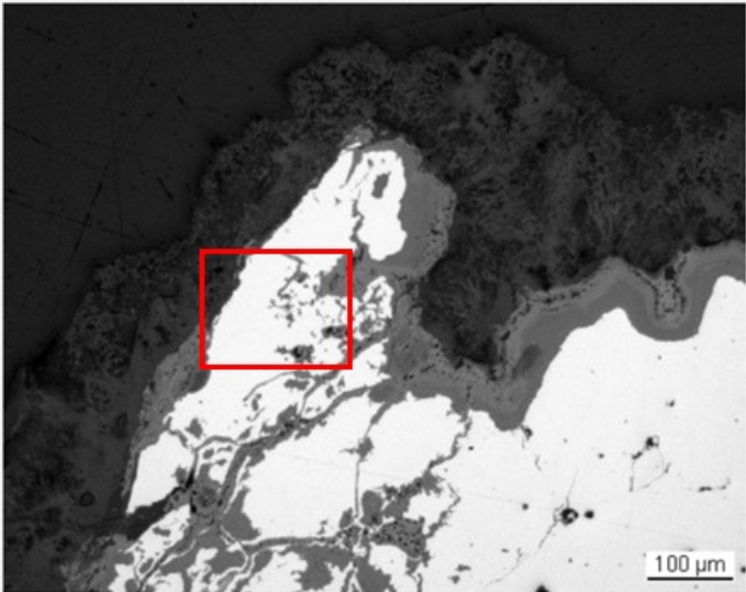
Fig. 4: Micrograph of the metal sample from Fig. 3 (detail), unetched, bright field. From bottom right to top left we observe: the metal (in white) with porosity (in black) and the corrosion layer (in light and dark-grey). The micrograph of Fig. 5 is marked by a rectangle,
