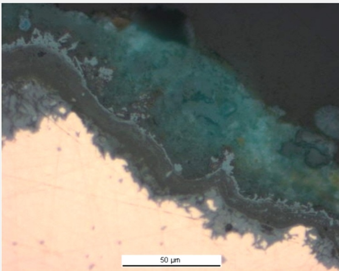
Fig. 7: Micrograph of the metal sample from Fig. 4 (detail) and corresponding to the stratigraphy of Fig. 10, unetched, bright field. Stratigraphy of the corrosion crust: inner light grey layer (CP3), intermediate dark grey layer with a light grey rim (CP2) and outer grey-green layer (CP1),
