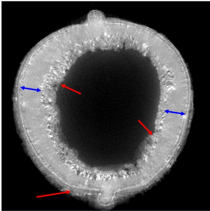
Fig. 11: X-ray tomography by cross section of the crown showing a dense and non-porous metal core (blue arrows). The corrosion products however are porous (red arrows). The external limit is visible as a fine line preserved under corrosion layers,
