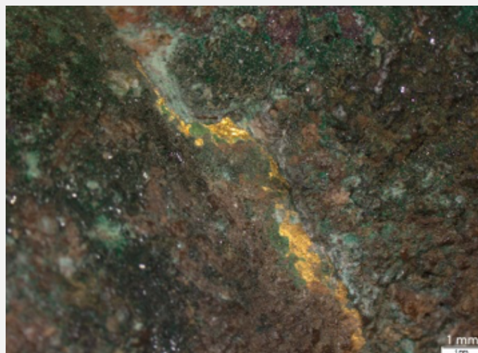
Fig. 3: Remains of foil-gilding on the corroded surface,
