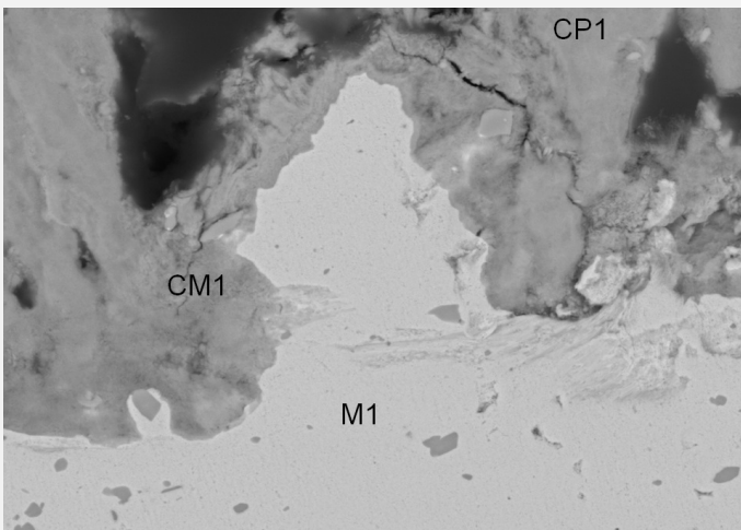
Fig. 8: SEM image (BSE mode) of a detail of the cross-section of the corroded lead came. The area in light grey is the metal, the corrosion is in darker grey with a blurred appearance. Sb-dots are dark grey. Corrosion progresses around them, without mineralising them,
