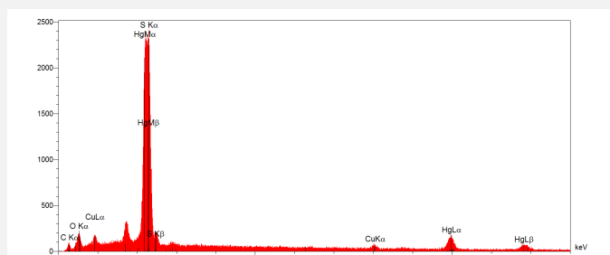
Fig. 12: EDS analysis of the red surface pigment from a surface sample. Method of analysis: SEM-EDS, Lab of Electronic Microscopy and Microanalysis, IMA (Néode), HEI Arc,
