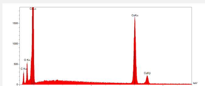
Fig. 11: EDS analysis of the green corrosion layer that has filled the structural void (Fig. 4). Method of analysis: SEM-EDS, Lab of Electronic Microscopy and Microanalysis, IMA (Néode), HEI Arc,
